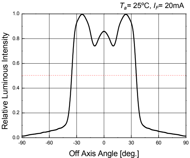
Directivity
