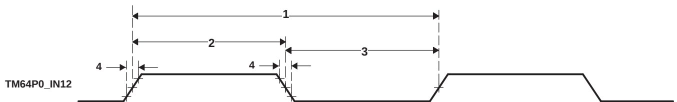
Figure 6-40. Timer Timing
