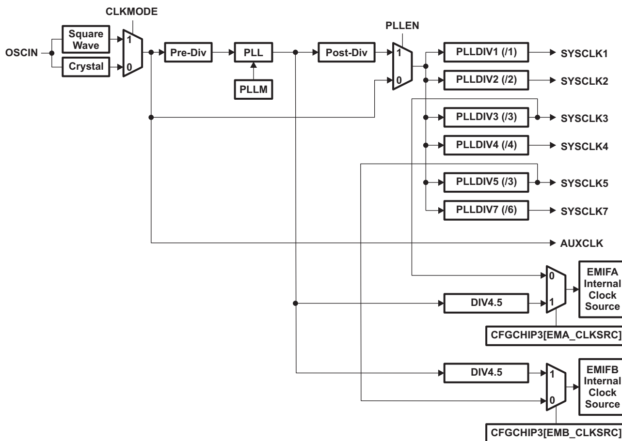
Figure 6-9. PLL Topology
