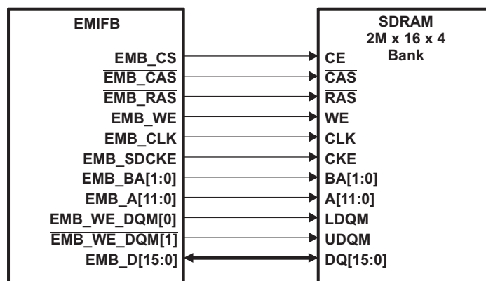
Figure 6-17. EMIFB to 2\text{M} \times 16 \times 4 bank SDRAM Interface
