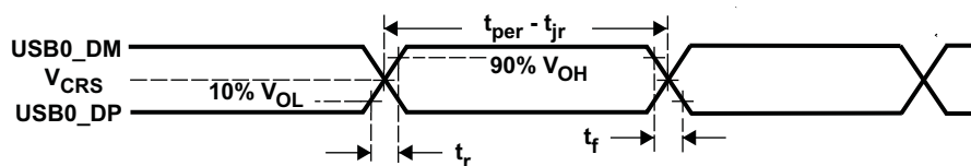
Figure 6-46. USB0 Integrated Transceiver Interface Timing
