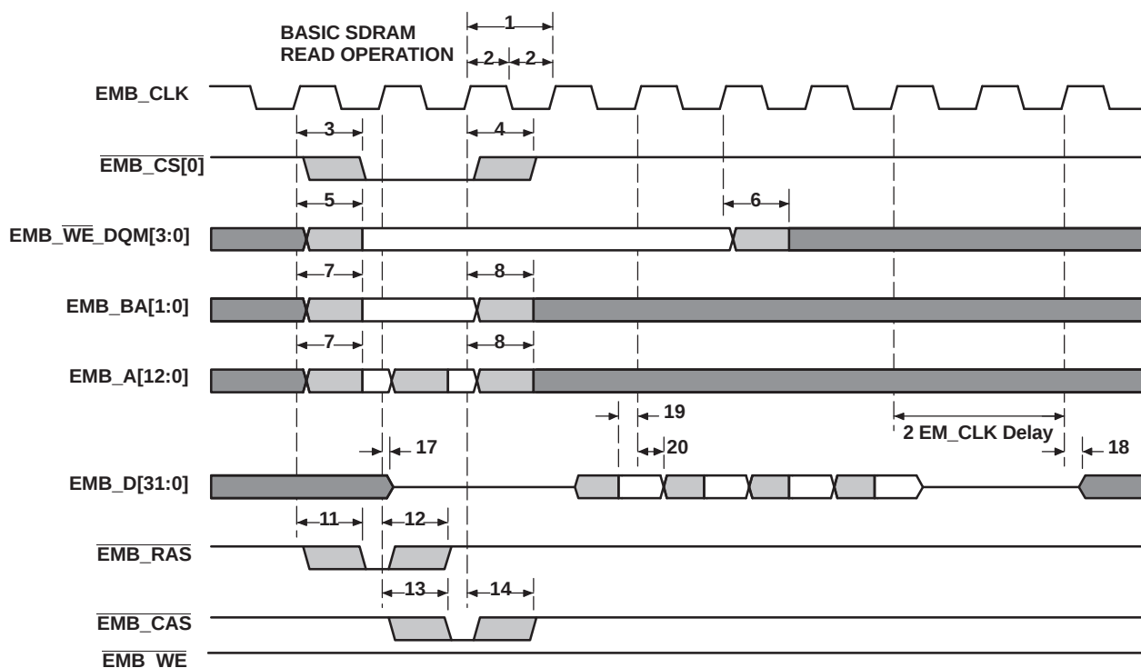
Figure 6-20. EMIFB Basic SDRAM Read Operation
