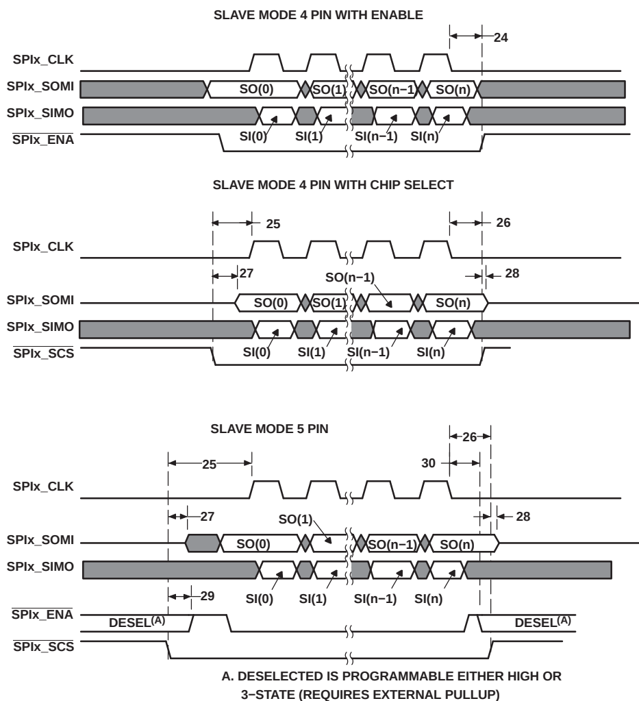
Figure 6-34. SPI Timings—Slave Mode (4-Pin and 5-Pin)
