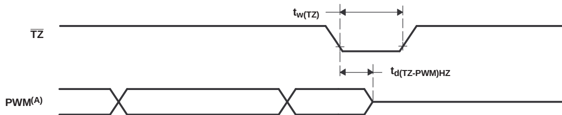
Figure 6-39. PWM Hi-Z Characteristics
