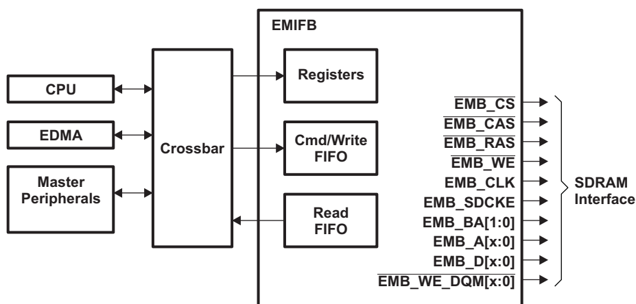
Figure 6-16. EMIFB Functional Block Diagram
