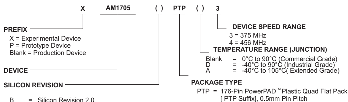
Figure 8-1. Device Nomenclature
