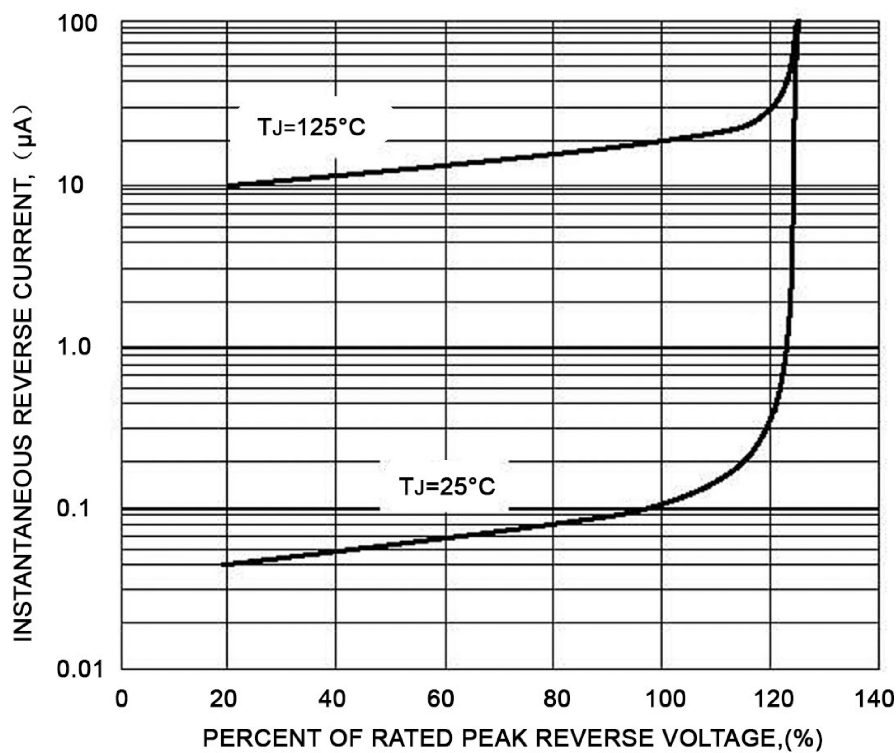
FIG.5-TYPICAL REVERSE CHARACTERISTICS
