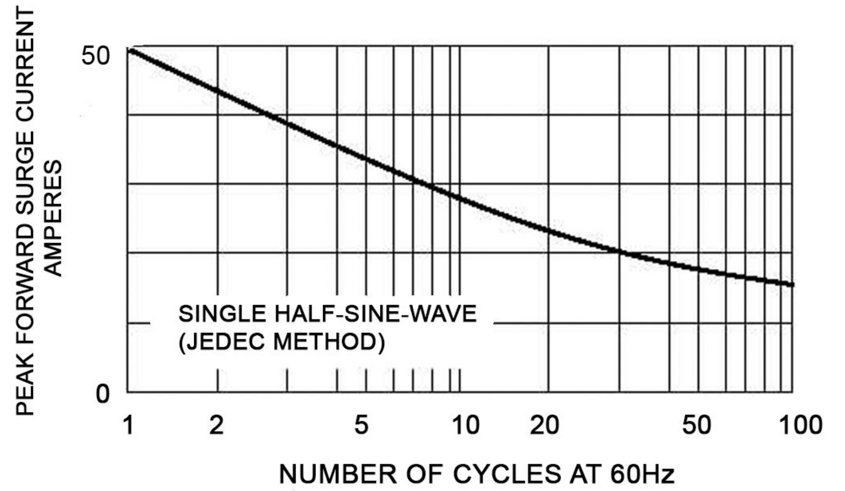
FIG.2-MXIMUM NON-REPETITIVE SURGE CURRENT
