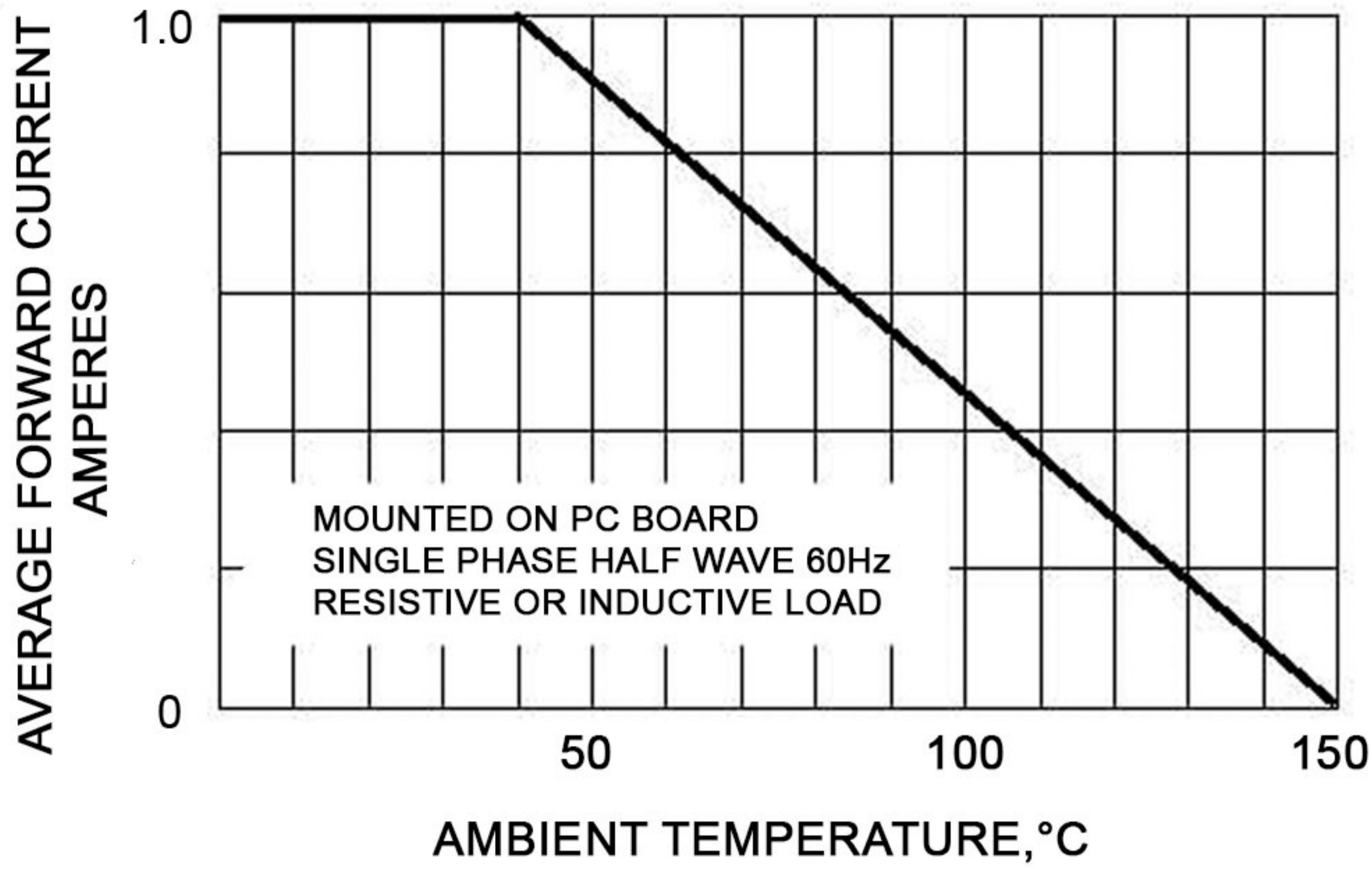
FIG.1-FORWARD CURRENT DERATING CURVE
