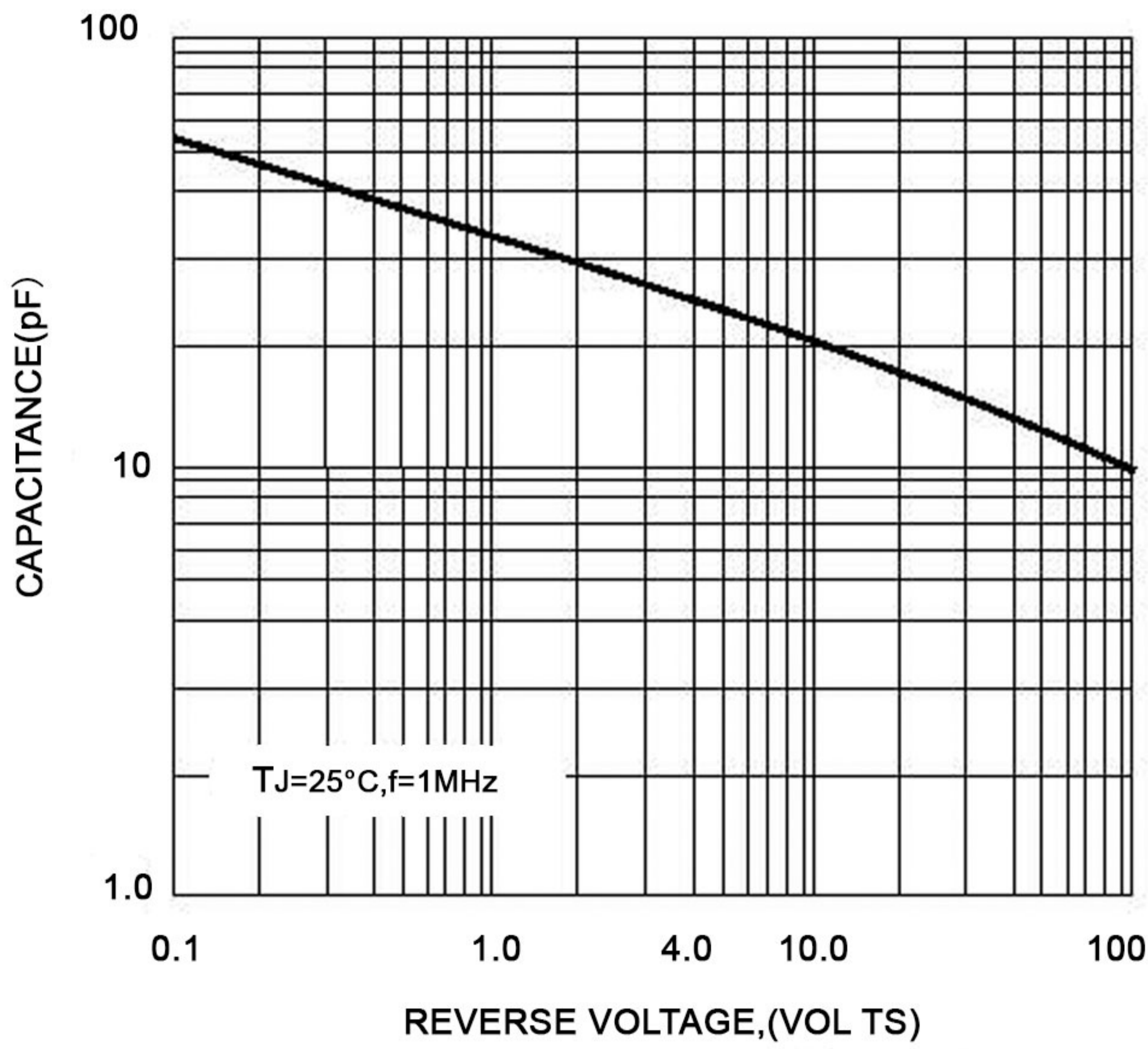
FIG.3-TYPICAL JUNCTION CAPACITANCE
