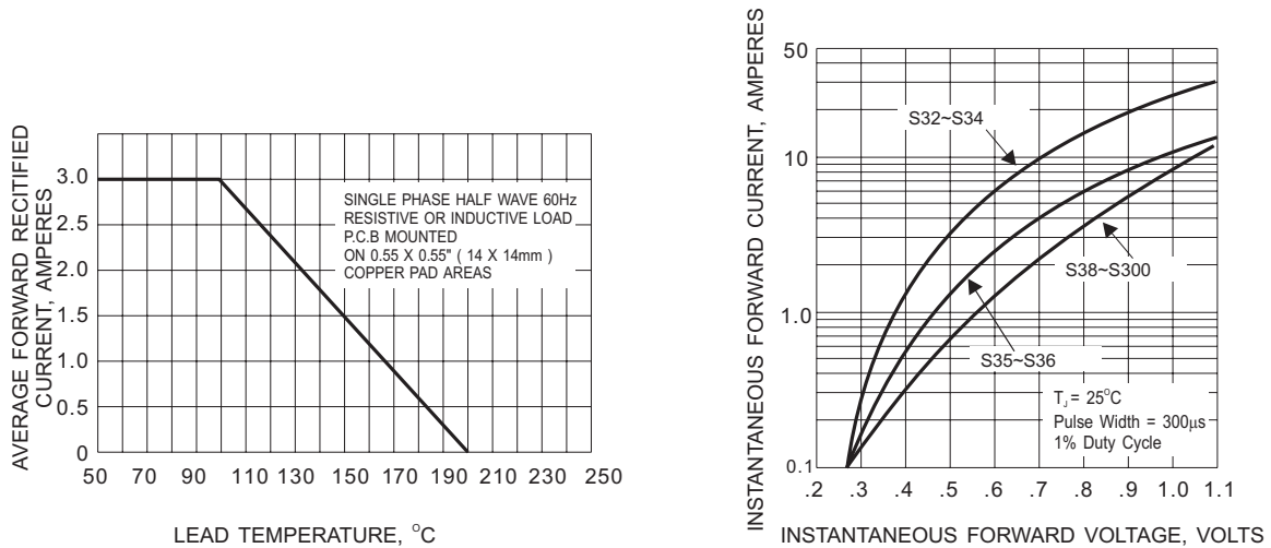
Fig.1- FORWARD CURRENT DERATING CURVE
