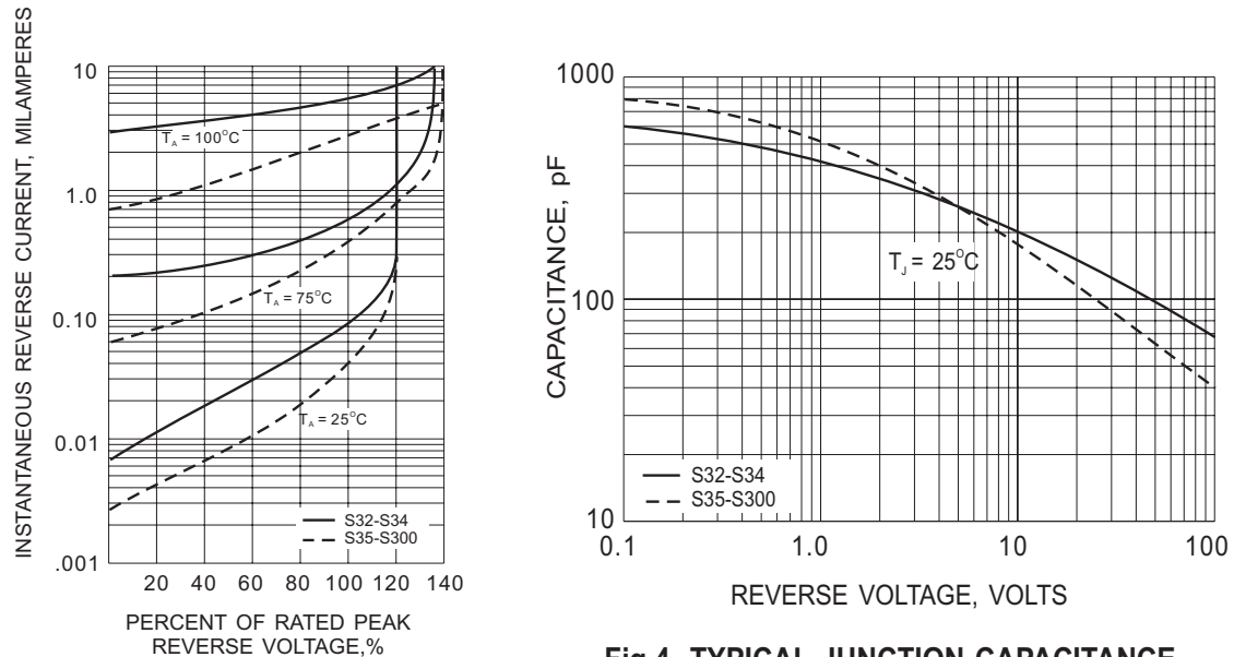
Fig.3- TYPICAL REVERSE CHARACTERISTIC
