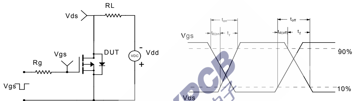
Resistive Switching Test Circuit &amp; Waveforms
