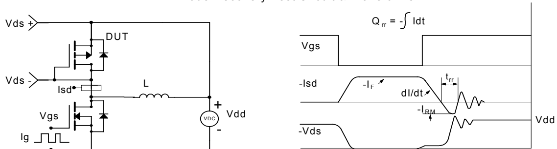
Diode Recovery Test Circuit &amp; Waveforms
