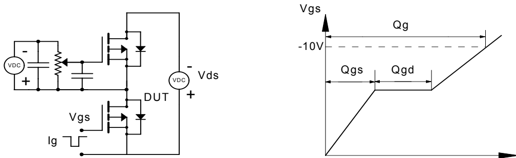
Gate Charge Test Circuit &amp; Waveform
