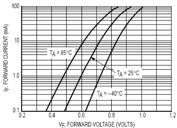
Figure 1. Forward Voltage
