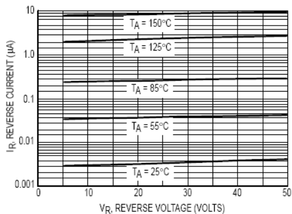
Figure 2. Leakage Current
