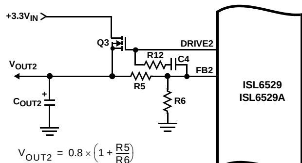
FIGURE 5. OUTPUT VOLTAGE SELECTION OF THE LINEAR
