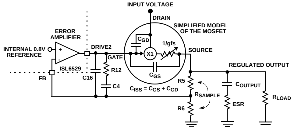
FIGURE 7. FIGURE A. SIMPLIFIED DIAGRAM OF THE LINEAR VOLTAGE REGULATOR
