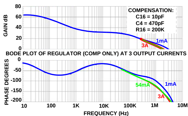
FIGURE 12. LOOP RESPONSE WITH COMPENSATION NETWORK ONLY
