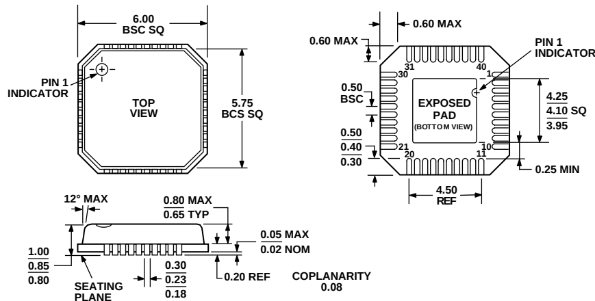
Figure 47. 40-Lead Lead Frame Chip Scale Package [LFCSP] 6 mm x 6 mm Body (CP-40) Dimensions shown in millimeters
