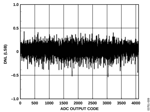
Figure 8. Typical DNL
