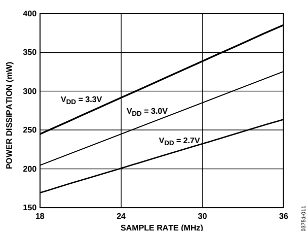
Figure 10. Power Curves
