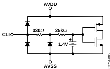
Figure 4. CLI (Pin 25)
