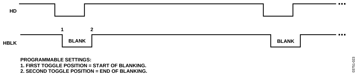
Figure 22. Horizontal Blanking (HBLK) Pulse Placement
