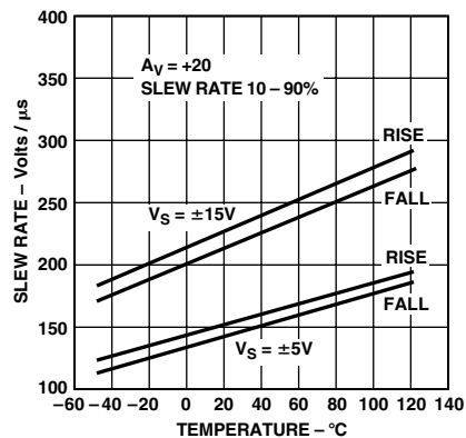
Figure 19. Slew Rate vs. Temperature
