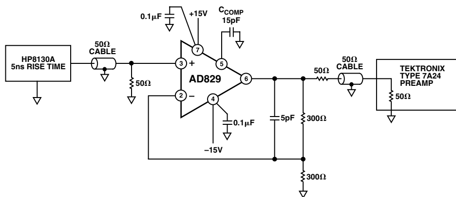
Figure 22a. Follower Connection. Gain = +2
