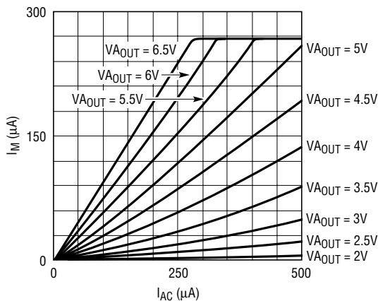
Multiplier Current
