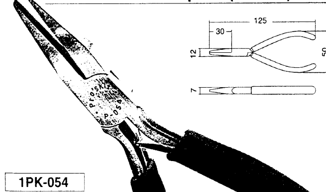
5" Flat nose plier (125mm)
