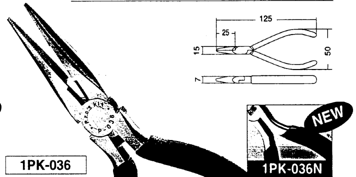
5" Long nose plier (125mm)
