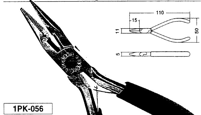
4.5" Long nose plier (110mm)
