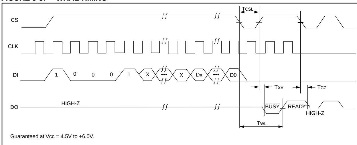
FIGURE 3-8: WRAL TIMING
