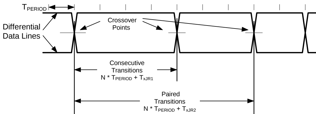
Figure 8-5. Differential Data Jitter
