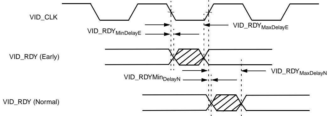
Figure 6-12. MPEG Timing
