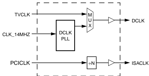
Figure 2-4. CS5530A Clock Generation
