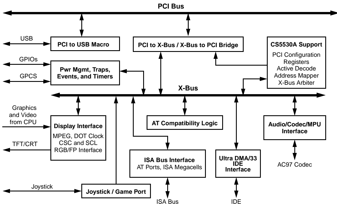
Figure 1-1. Block Diagram
