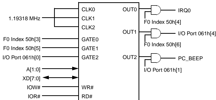
Figure 4-14. PIT Timer
