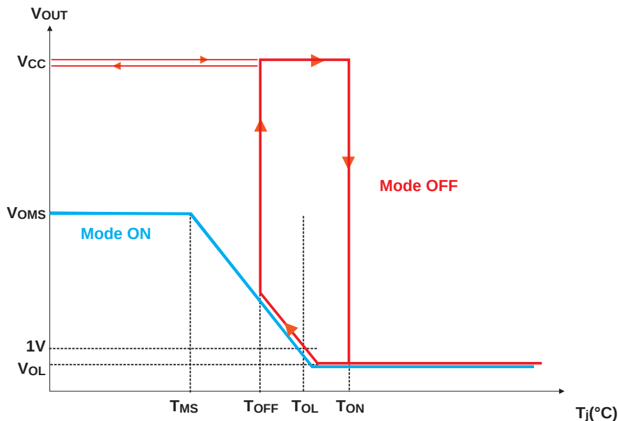
Fig. 7: OUT voltage versus junction temperature.
