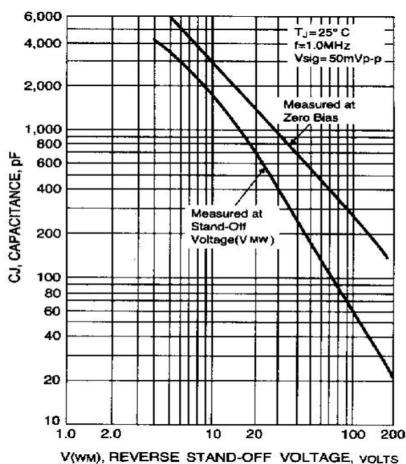
Fig. 4-TYPICAL JUNCTION CAPACITANCE
