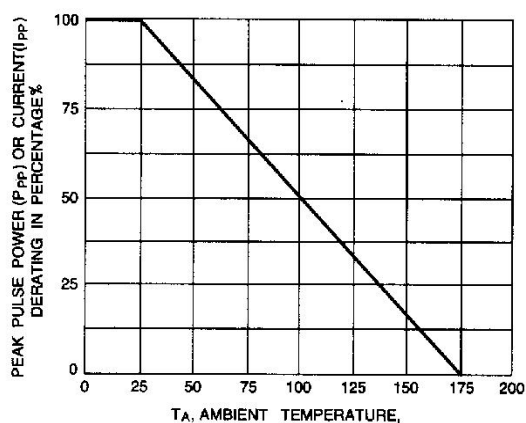
Fig. 2-PULSE DERATING CURVE
