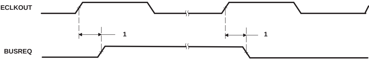
Figure 30. BUSREQ Timing
