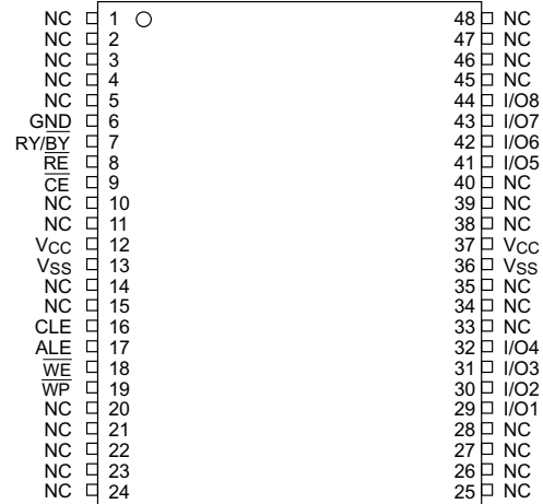
Figure 1. Pinout
