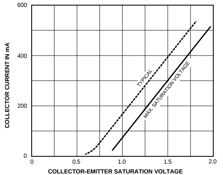
SATURATION VOLTAGE AS A FUNCTION OF COLLECTOR CURRENT
