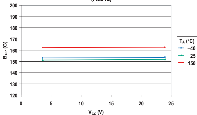
Operate Point versus Supply Voltage (A3242)
