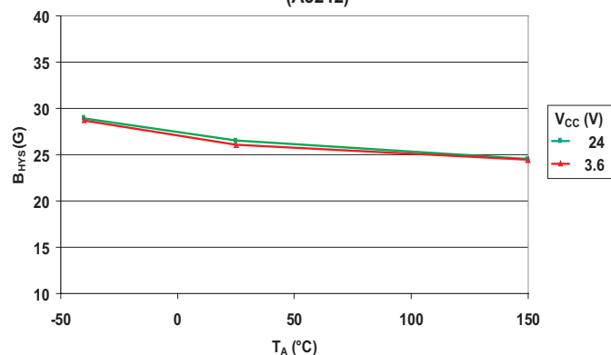
Hysteresis versus Ambient Temperature (A3242)
