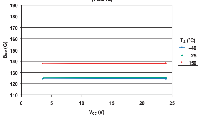
Release Point versus Supply Voltage (A3242)
