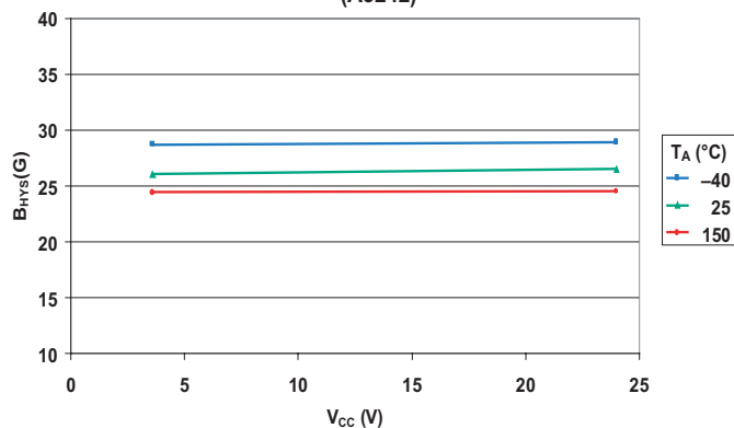
Hysteresis versus Supply Voltage (A3242)
