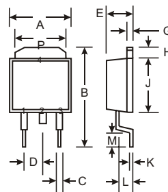
TO-252 / DPAK
