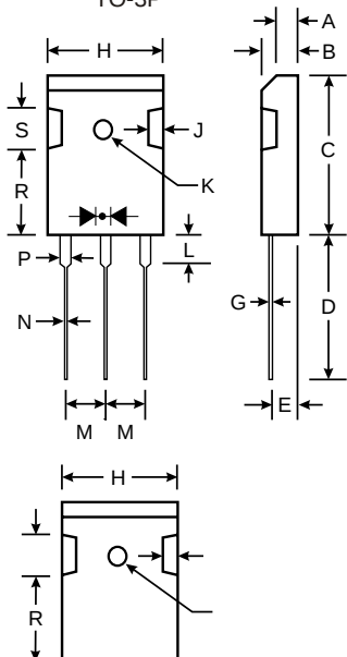
TO-3P
