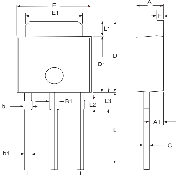
TO-251
