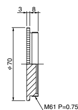
CAP (SUPPLIED)
