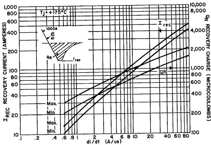
5. REVERSE RECOVERY CHARACTERISTICS
