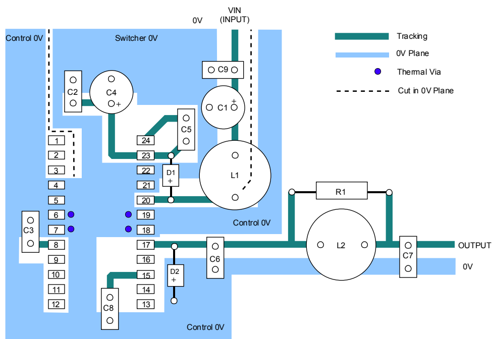
PCB Layout Diagram
