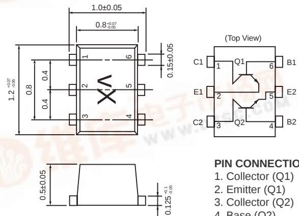
Package Outline TD (TOP VIEW)
