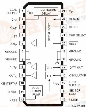
A8904SLB (SOIC)
