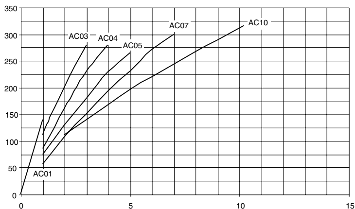
Temperature Rise
