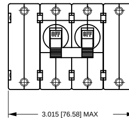
4-POLE (AB4)
