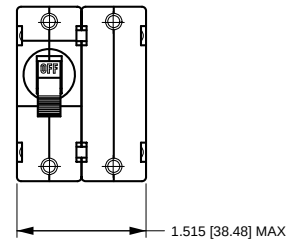
2-POLE (AB2)
