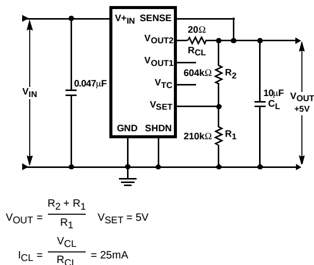
FIGURE 8. POSITIVE REGULATOR WITH CURRENT LIMIT
