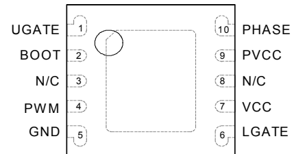
ISL6594ACR, ISL6594BCR (10L 3x3 DFN) TOP VIEW
