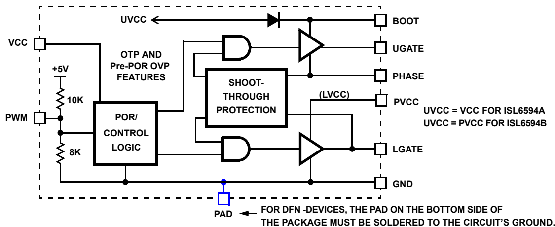
ISL6594A AND ISL6594B
