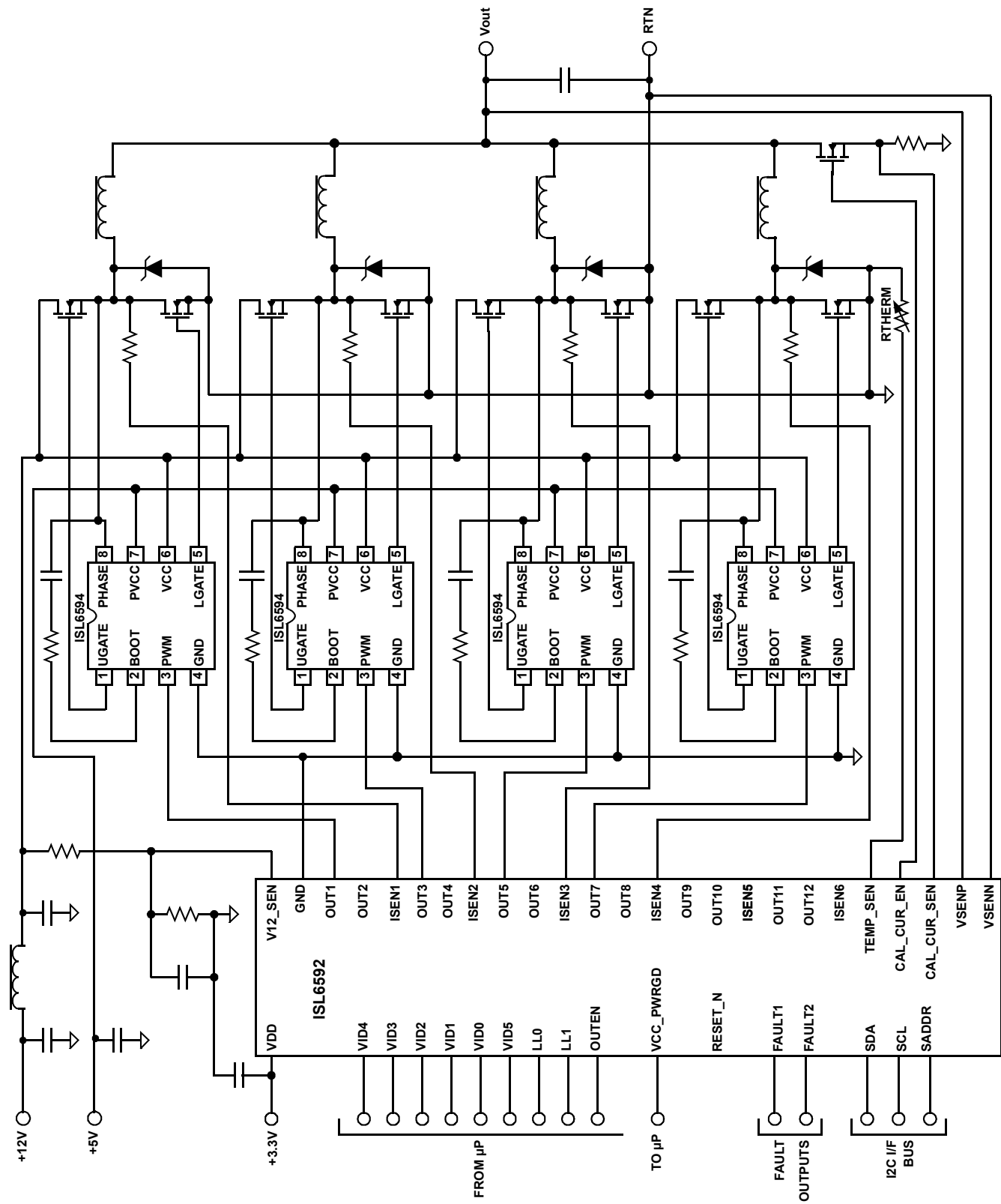
Typical Application - 4 Channel Converter Using ISL6592 and ISL6594A Gate Drivers
