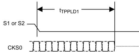
FIGURE 26. PLL Power-Down Time
