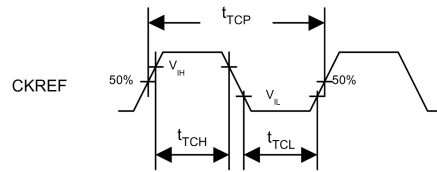
FIGURE 18. LVCMOS Clock Parameters
