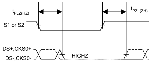
FIGURE 27. Serializer Enable and Disable Time
