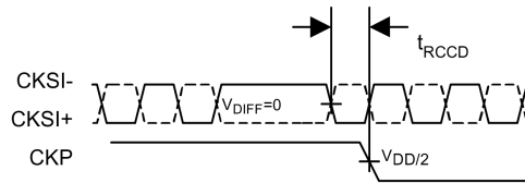
FIGURE 22. Deserializer Clock Propagation Delay
