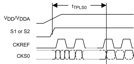
FIGURE 20. Serializer PLL Lock Time
