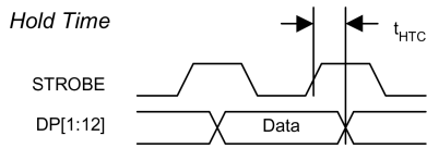
FIGURE 17. Serial Setup and Hold Time
