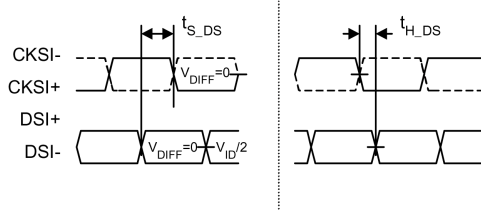
FIGURE 23. Differential Input Setup and Hold Times
