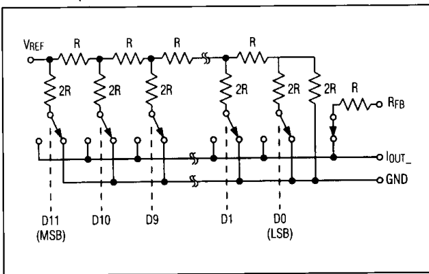
Figure 1. Simplified D/A Circuit for 1/4 of MAX514
