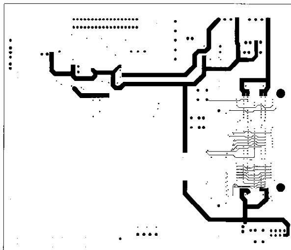
Figure 26. Power Plane 2
