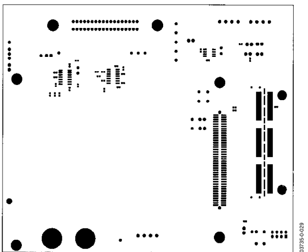
Figure 31. Top Mask
