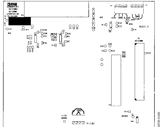
Figure 32. Top Silkscreen
