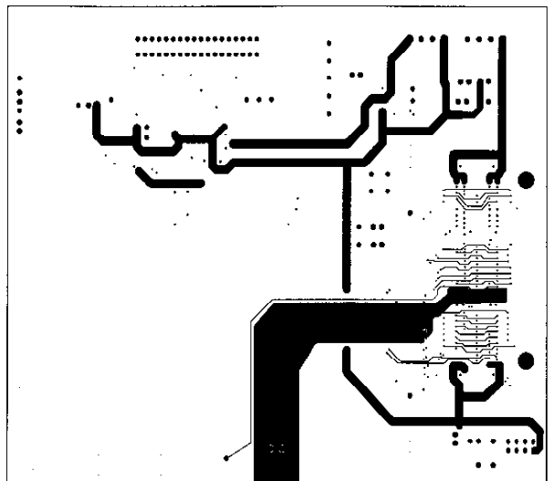
Figure 25. Power Plane 1
