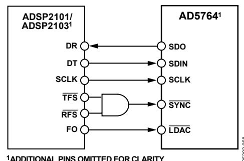
Figure 40. AD5764 to ADSP2101/ADSP2103 Interface
