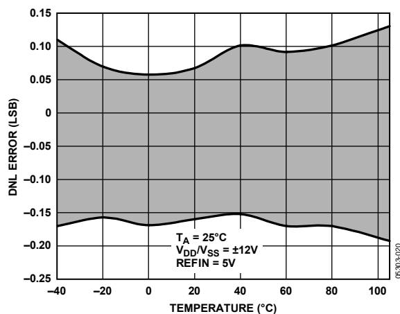
Figure 14. AD5764 Differential Nonlinearity Error vs. Temperature, V_{DD}/V_{SS} = \pm 12V
