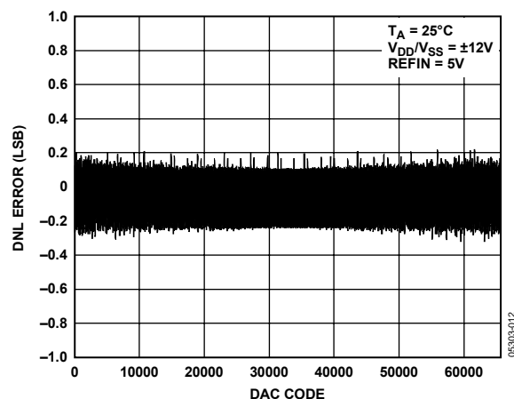
Figure 10. AD5764 Differential Nonlinearity Error vs. Code, V_{DD}/V_{SS} = \pm 12\text{ V}
