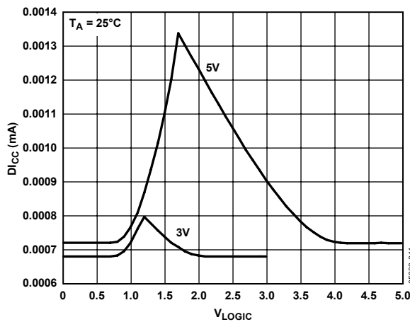
Figure 24. D_{LCC} vs. Logic Input Voltage
