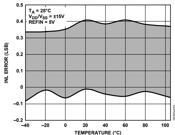
Figure 11. AD5764 Integral Nonlinearity Error vs. Temperature, V_{DD}/V_{SS} = \pm 15\text{ V}
