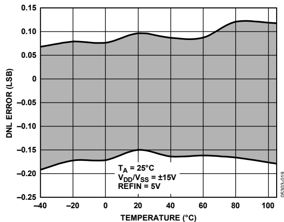
Figure 13. AD5764 Differential Nonlinearity Error vs. Temperature, V_{DD}/V_{SS} = \pm 15V
