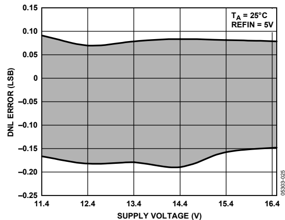
Figure 16. AD5764 Differential Nonlinearity Error vs. Supply Voltage
