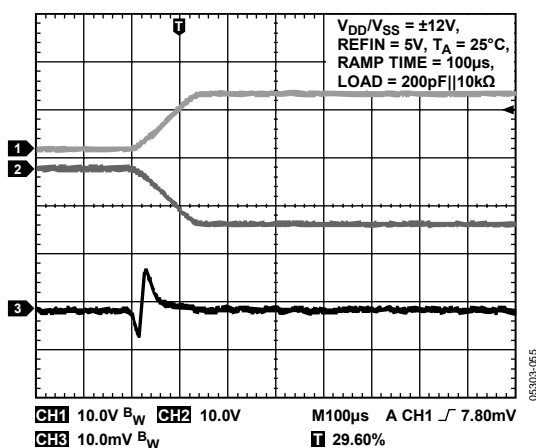
Figure 30. V_{OUT} vs. V_{DD}/V_{SS} on Power-Up
