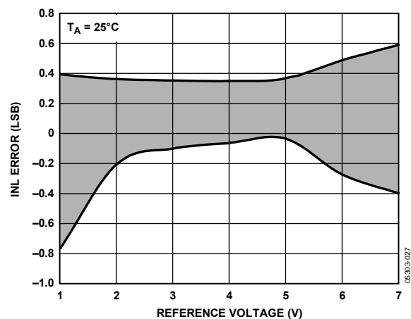
Figure 17. AD5764 Integral Nonlinearity Error vs. Reference Voltage, V_{DD}/V_{SS} = \pm 16.5V
