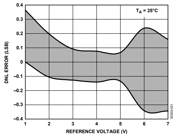
Figure 18. AD5764 Differential Nonlinearity Error vs. Reference Voltage, V_{DD}/V_{SS} = \pm 16.5V
