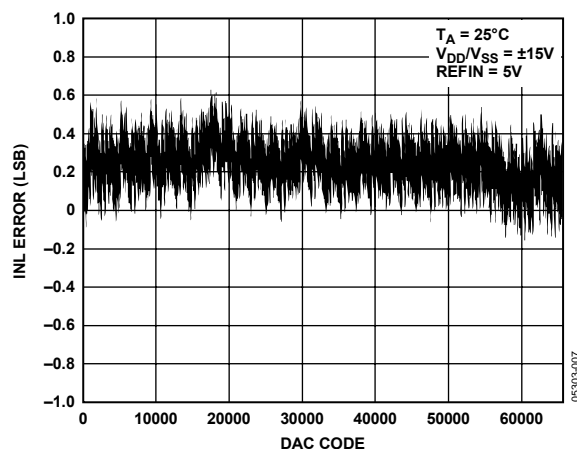
Figure 7. AD5764 Integral Nonlinearity Error vs. Code, V_{DD}/V_{SS} = \pm 15\text{ V}
