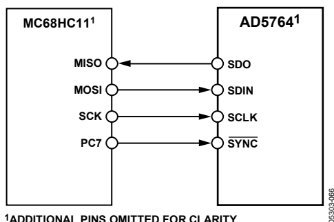
Figure 38. AD5764 to MC68HC11 Interface
