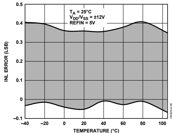
Figure 12. AD5764 Integral Nonlinearity Error vs. Temperature, V_{DD}/V_{SS} = \pm 12\text{ V}
