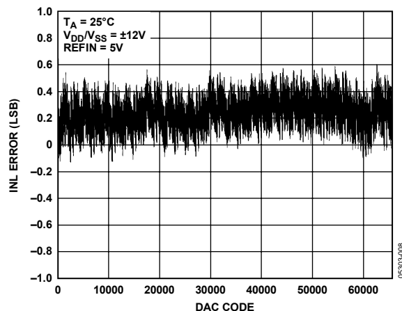
Figure 8. AD5764 Integral Nonlinearity Error vs. Code, V_{DD}/V_{SS} = \pm 12\text{ V}
