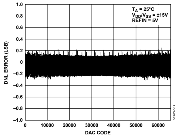
Figure 9. AD5764 Differential Nonlinearity Error vs. Code, V_{DD}/V_{SS} = \pm 15\text{ V}
