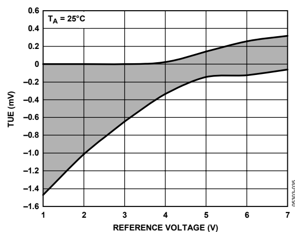
Figure 19. AD5764 Total Unadjusted Error vs. Reference Voltage, V_{DD}/V_{SS} = \pm 16.5\text{ V}
