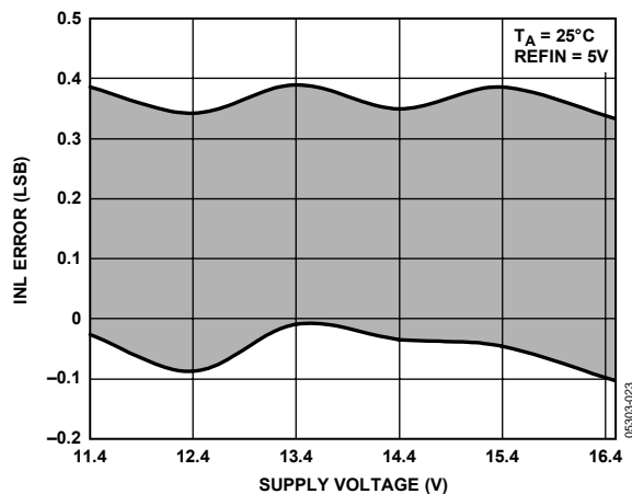
Figure 15. AD5764 Integral Nonlinearity Error vs. Supply Voltage
