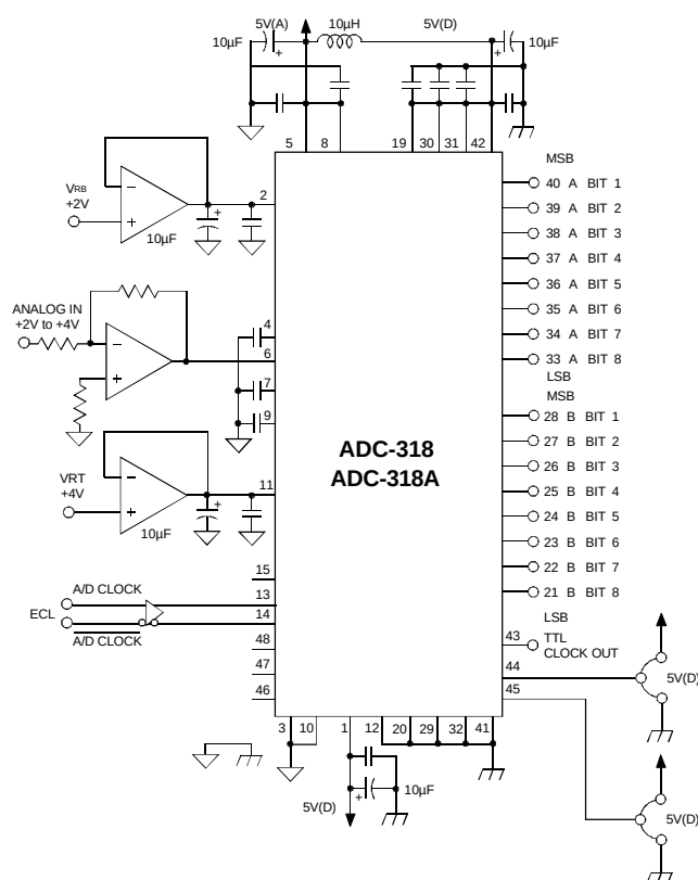
Figure 2-2: Two Power Supply Operation (ECL)
