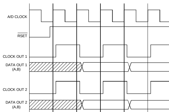
Figure 3-2: Straight Data Output (Select-Pin: DGND, 100MHz max. Clock Frequency)
