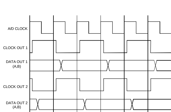
Figure 3-2: Straight Data Output (Select-Pin: DGND, 100MHz max. Clock Frequency)
