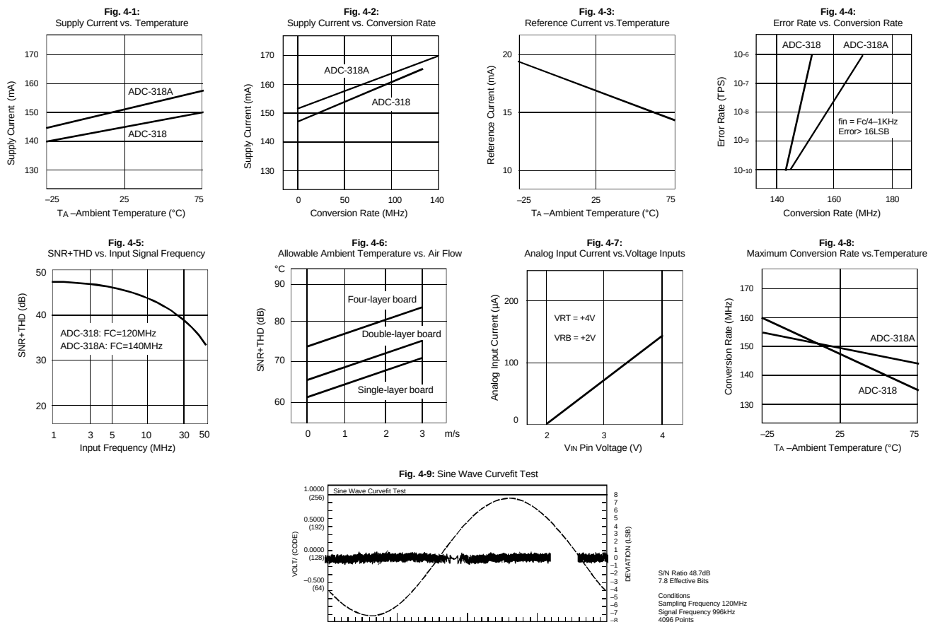
Figure 6: Typical Performance Curve
