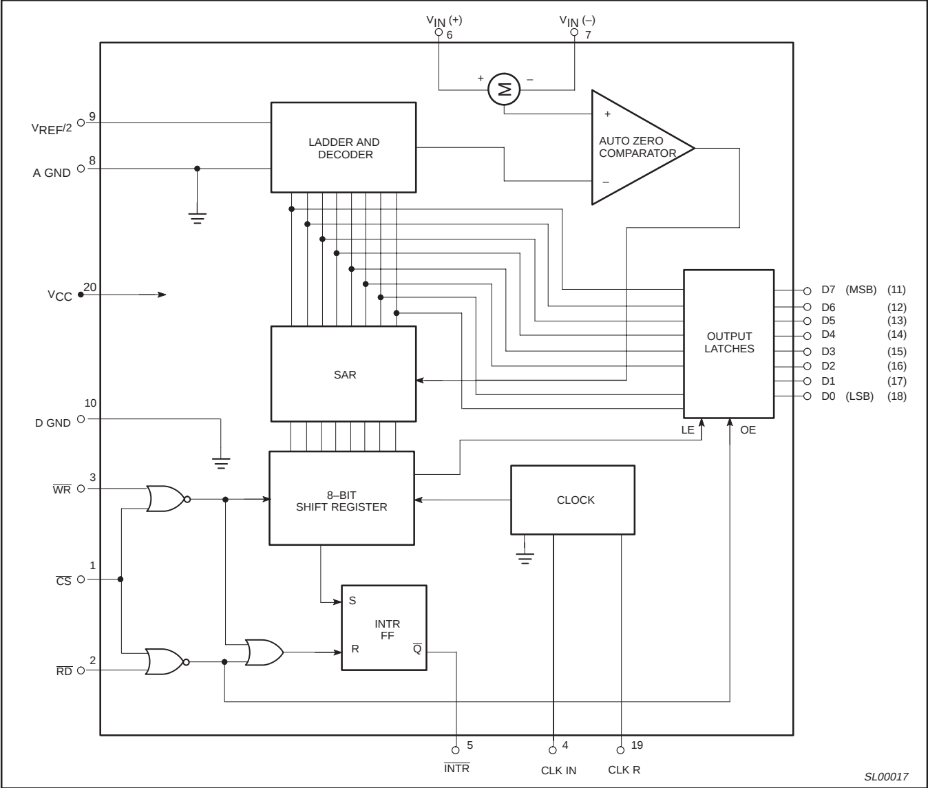
Figure 2. Block diagram
