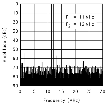
Intermodulation Distortion (IMD)
