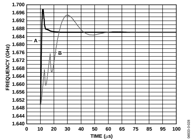
Figure 16. A) Lock Time in Fast-lock Mode. Fast Counter = 150, Low Spur Mode: a 1649.7 MHz to 1686.8 MHz Frequency Jump. Final Loop Bandwidth = 60 kHz
