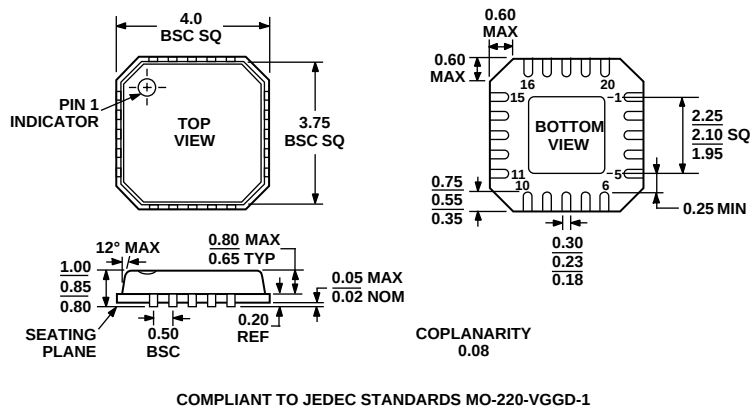
Figure 27. 20-Lead Lead Frame Chip Scale Package [LFCSPP] 4 mm × 4 mm Body, (CP-20) Dimensions shown in millimeters
