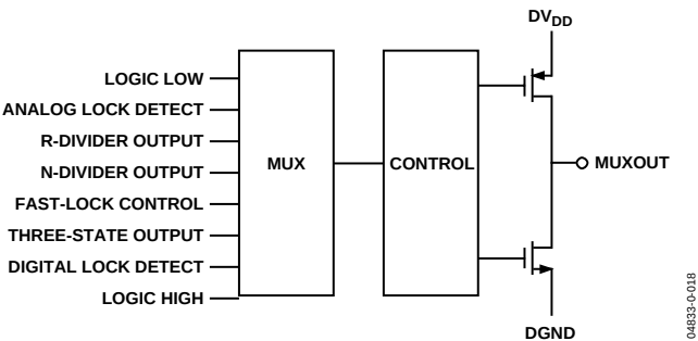
Figure 21. MUXOUT Schematic
