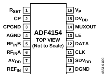
Figure 3. TSSOP Pin Configuration
