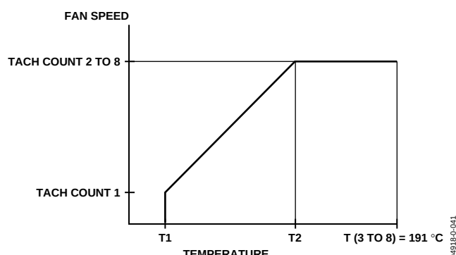
Figure 42. Programming Two Points on the Look-Up Table
