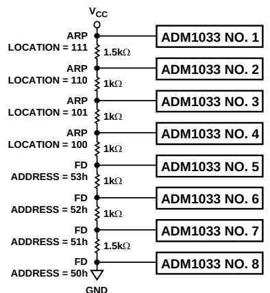
Figure 17. Setting Up Multiple ADM1033 Addresses
