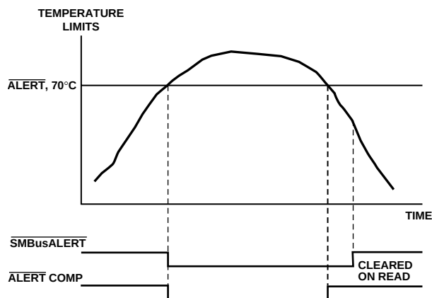
Figure 31. How ALERT Comparator and SMBusALERT Outputs Work
