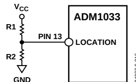
Figure 16. Bootstrapping the LOCATION Input
