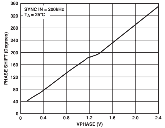
TPC 4. Clock Phase Shift vs. Phase Voltage
