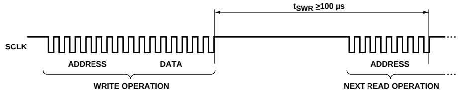
Figure 32. Timing between write and read commands.
