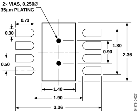
Figure 27. 3 mm × 3 mm LFCSP Pad Pattern (Dimensions in mm)
