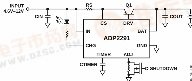
Figure 1. Basic Circuit Configuration
