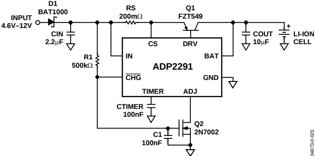
Figure 23. Self-Termination Circuit
