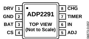
Figure 2. 8-Lead MSOP
