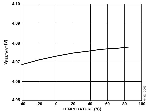
Figure 9. Restart Threshold
