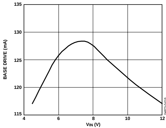
Figure 16. Base Drive vs. Input Voltage
