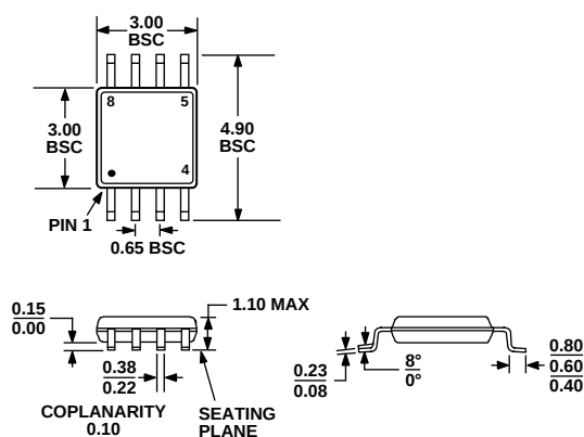
Figure 29. 8-Lead MSOP Package (RM-8) Dimensions Shown in Millimeters
