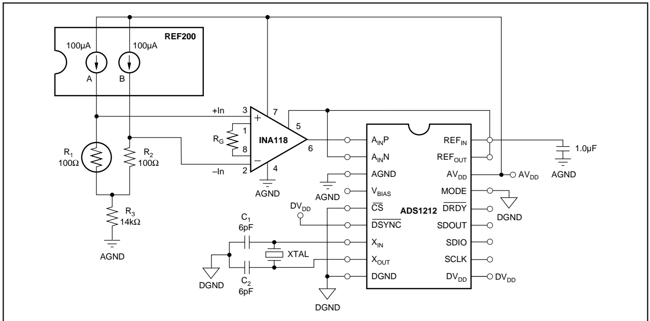
FIGURE 39. PT100 Interface.
