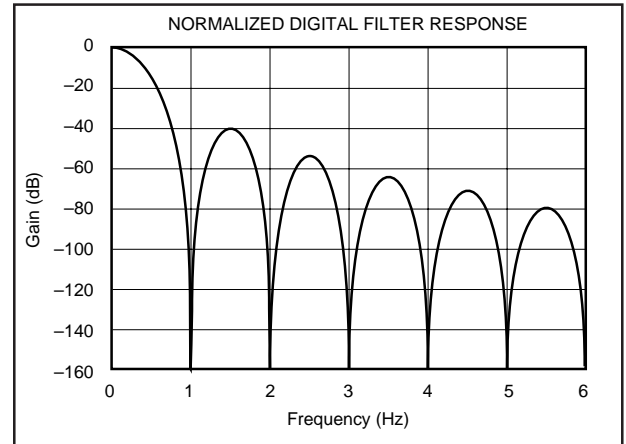
FIGURE 1. Normalized Digital Filter Response.
