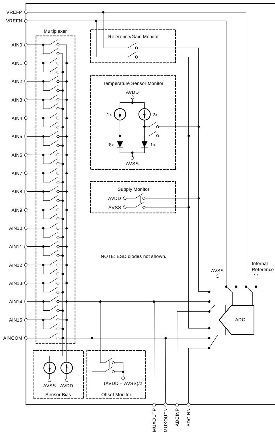
Figure 35. Input Multiplexer
