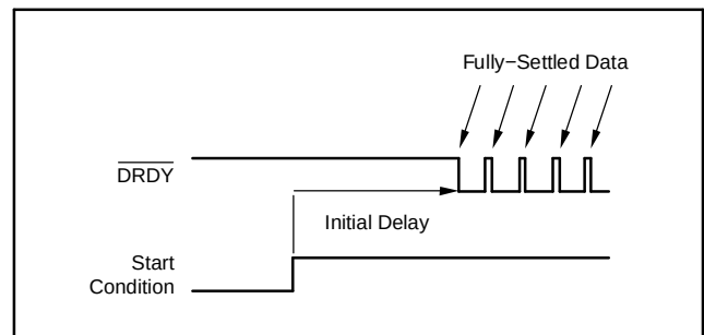
Figure 55. Start Condition to First Data
