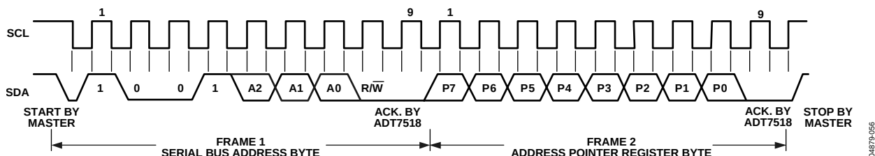
Figure 56. I²C—Writing to the Address Pointer Register to Select a Register for a Subsequent Read Operation
