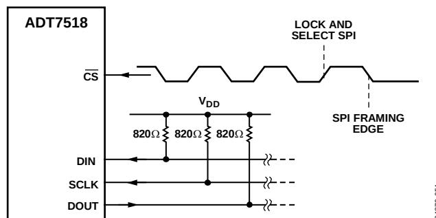
Figure 55. Typical SPI Interface Connection
