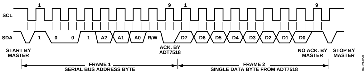
Figure 58. I²C—Reading a Single Byte of Data from a Selected Register
