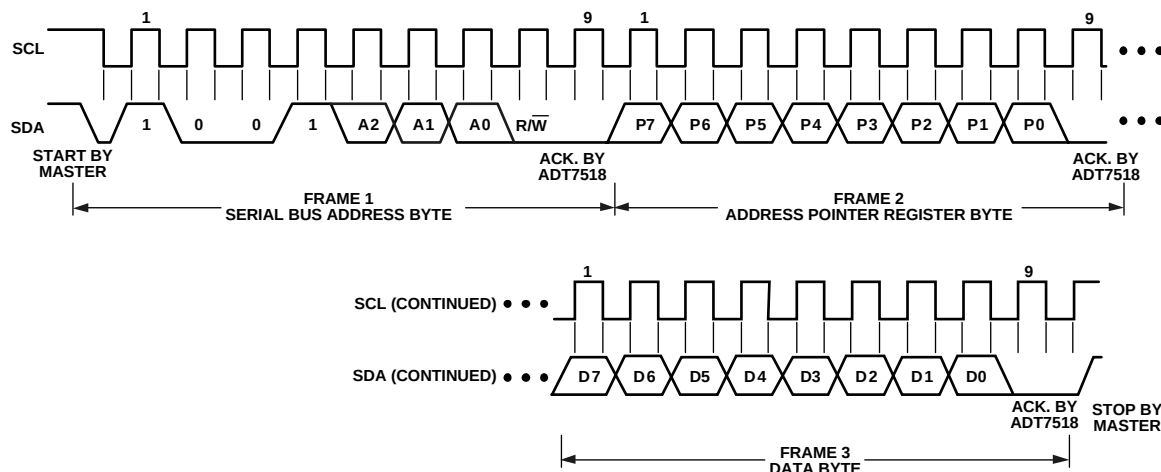
Figure 57. I²C—Writing to the Address Pointer Register Followed by a Single Byte of Data to the Selected Register
