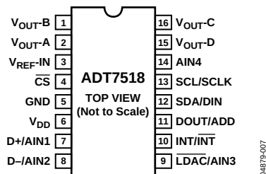
Figure 7. Pin Configuration QSOPT
