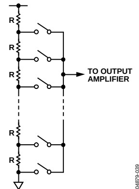
Figure 39. Resistor String
