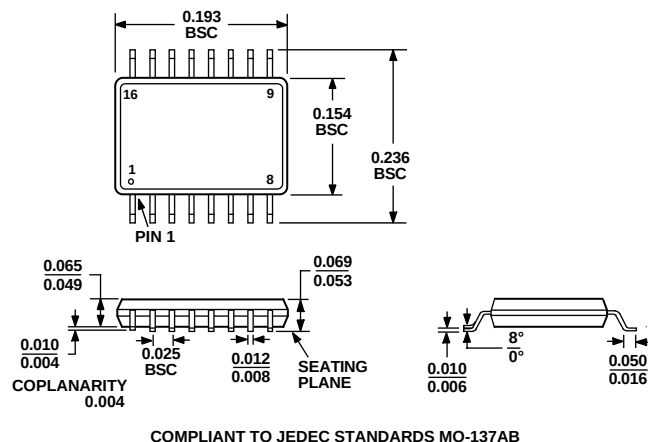
Figure 66. 16-Lead Shrink Small Outline Package [QSOP] (RQ-16) Dimensions in Inches
