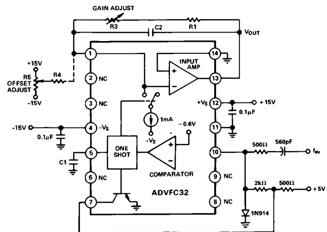
Figure 4. Connection Diagram for F/V Conversion, TTL Input
