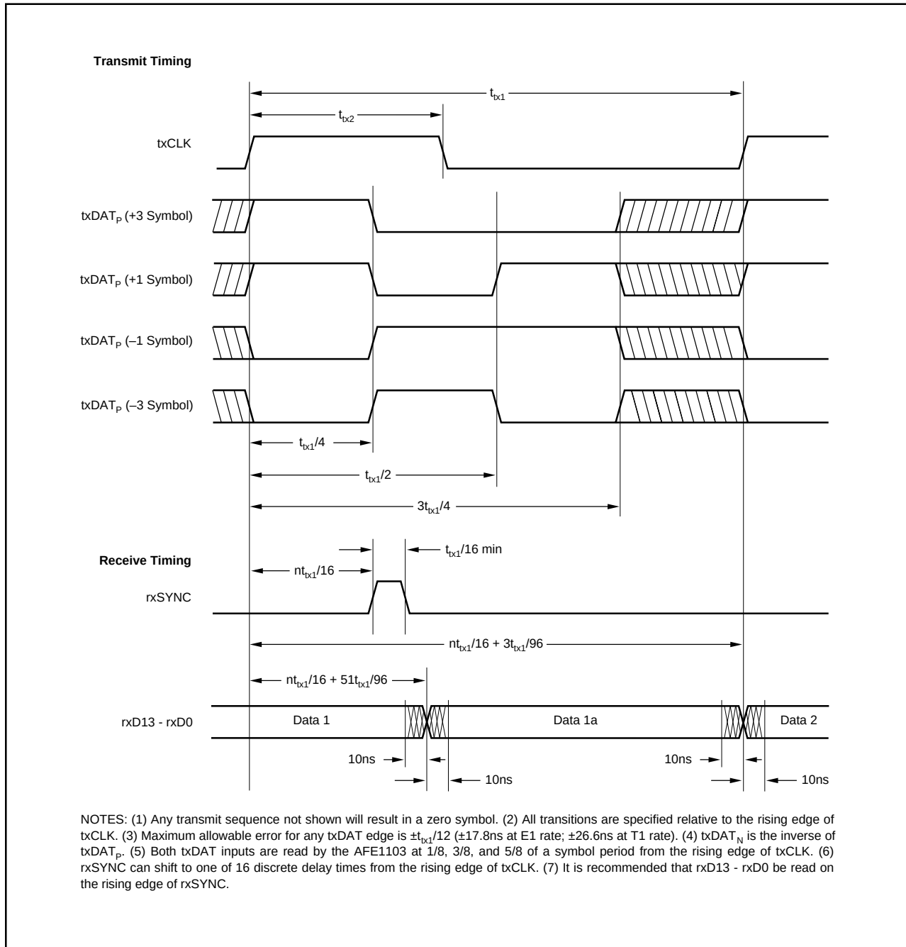
FIGURE 3. Timing Diagram.
