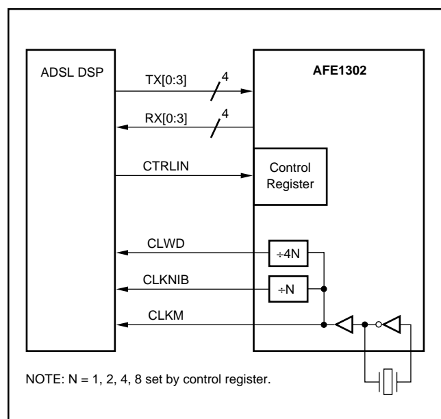
FIGURE 1. AFE1302/DSP Interface.
