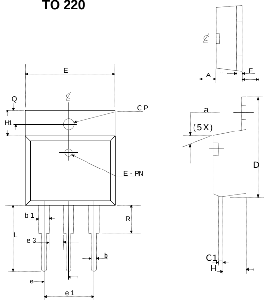
TO 220
