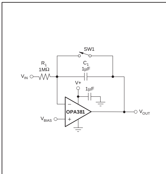
Figure 15. Precision Integrator
